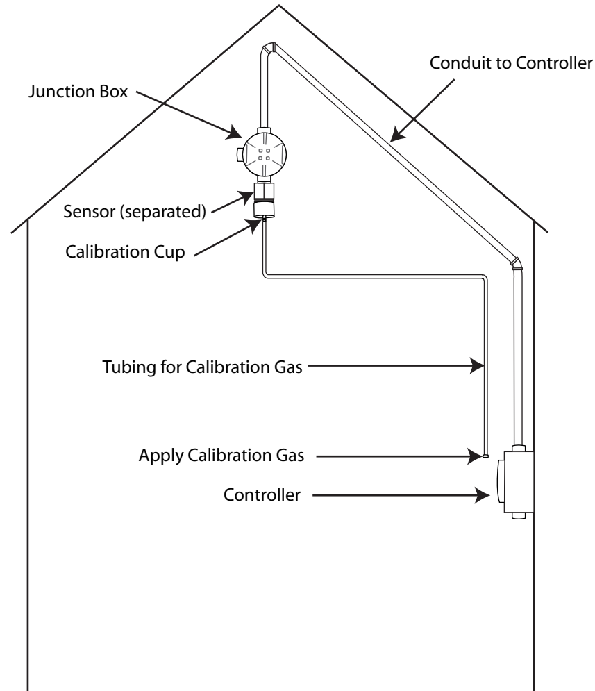
Figure 2: Locate Sensor/Controller - Separated
