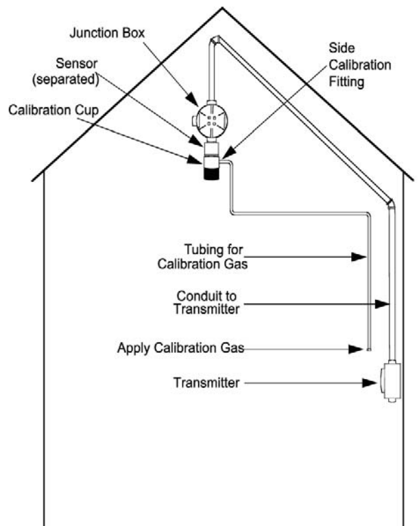
Figure 3: Locating Sensor
